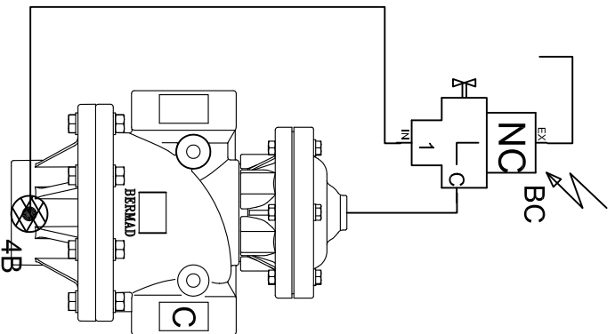
Angle pattern 350 series valve using S-390-3W-NC-24VAC-BO solenoid
