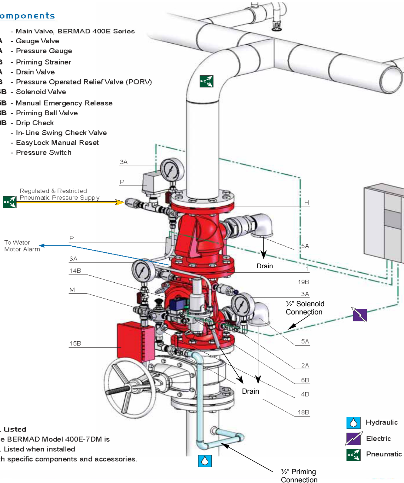
Figure 1: Installation Drawing
