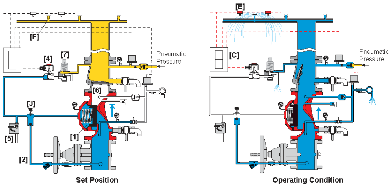
Figure 2: Operation Drawing
